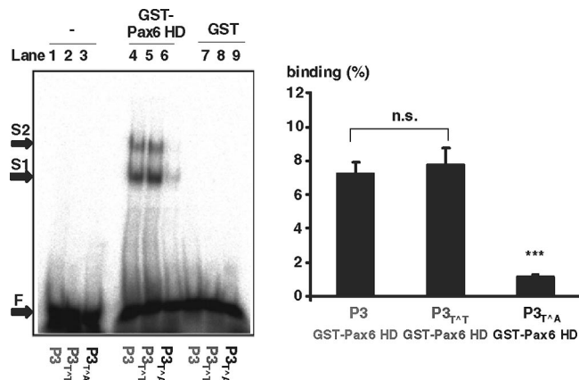
Figure 5. Binding of the Pax6 HD to the modified P3 sites. Left: electrophoretic mobility shift assay of the GST-Pax6 HD fusion protein with the modified oligonucleotides. The labeled oligonucleotides P3 , P3 T ^ T and P3 T ^ A were incubated with 250 ng of GST-Pax6 HD. GST was incubated with the indicated oligonucleotides as a specific control (Lanes 7–9). F = free probe; S1 and S2 = shifted probes; the two bands appearing for shifted probes were interpreted as homodimeric (S2) and monomeric (S1) binding complexes of HD with the probe. [16] Sequences of the oligonucleotides used in the gel retardation analysis are shown in the Exp. Sect. Right: Densitometric measurement of the percentage of binding of the indicated probes by the Pax6 HD using the PhosphorImager. Values are means ( \pm SEM) of four independent experiments statistically evaluated by Student's t test ***, p < 0.001.
