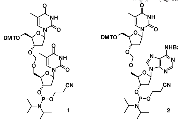
Figure 2. Formacetal-linked dinucleotide building blocks T ^ T ( 1 ) and T ^ A ( 2 ) for oligonucleotide solid-phase synthesis.
