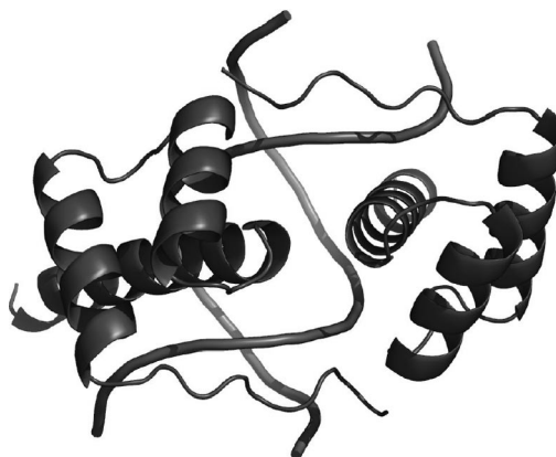
Figure 1. Binding of the HD of the protein paired from Drosophila as a dimer to an ideal P3 site TAATCTGATTA. [16] The Pax6 HD shows high sequence identity with the paired HD, and for the PAX6 HD a similar dimeric binding complex with P3 fragment can be expected. The recognition helix of HD interacts with the specific DNA motif ATTA.
