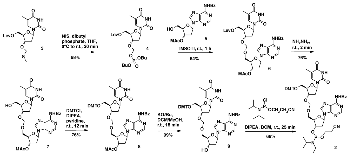
Scheme 1. Synthesis of the dinucleotide T A as phosphoramidite 2 ready to use in solid-phase oligonucleotide synthesis.
