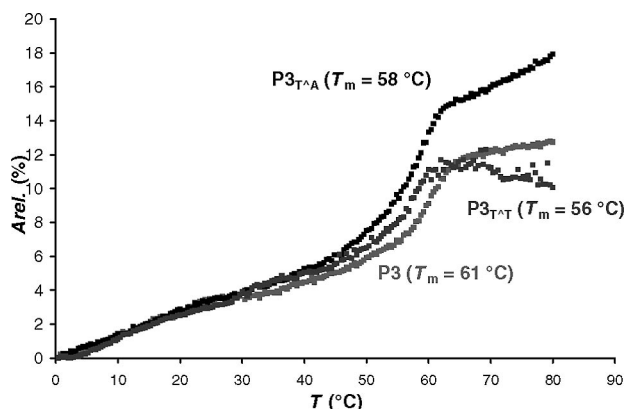
Figure 3. Temperature-dependent UV measurements of P3 , P3 T A and P3 T T measured in 10 mM phosphate buffer, pH = 7.0, 260 nm.
