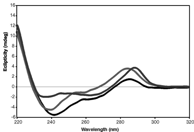
Figure 4. CD spectra of P3 T T and P3 T A compared to the native P3 oligomer, measured in 10 mM phosphate buffer, pH = 7.0.
